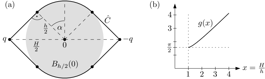
Figure 5: (a) The curve \hat{C} is the shortest curve enclosing B_{h/2}(0) and connecting q and -q . (b) A plot of the lower bound on geometric dilation depending on x = H/h .
