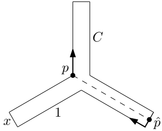
Figure 13: By decreasing x we can make the area of this closed curve arbitrarily small while h stays bounded.
