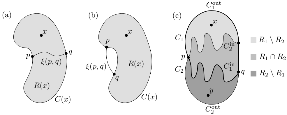
Figure 8: Impossible situations: (a) a shortest path \xi(p, q) crossing R(x) or (b) being a shortcut; (c) two crossing shortest cycles.
