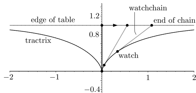
Figure 11: The tractrix, the curve of a watch on a table towed with its watchchain (the curve is symmetric about the y -axis).
