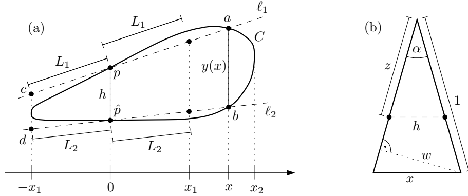
Figure 15: (a) Proving by contradiction that y(x) \leq h for every x in [x_1, x_2] . (b) In a thin isosceles triangle h/w \searrow 1/2 if \alpha \rightarrow 0 .
