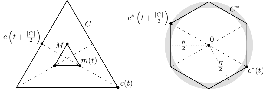
Figure 4: An equilateral triangle C , and the two curves C^* and M derived from C .
