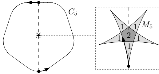
Figure 14: The midpoint curve of a rounded pentagon, constructed analogously to C_\Delta of Figure 9, has 5 cusps. It contains regions with winding number 2 and regions with winding number 1.
