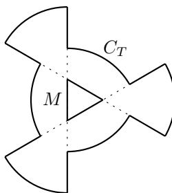
Figure 10: C_T consists of translation parts and circular arcs.
