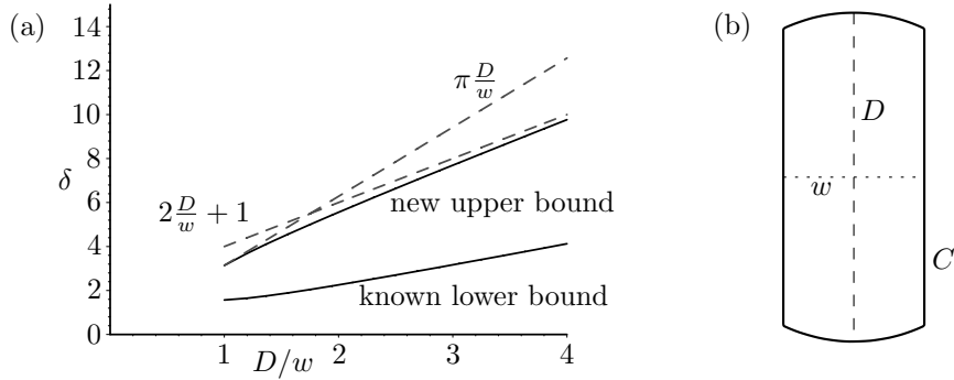
Figure 16: (a) A plot of the new upper bound on geometric dilation and the known lower bound. (b) The extremal set of Kubota's inequality (14).
