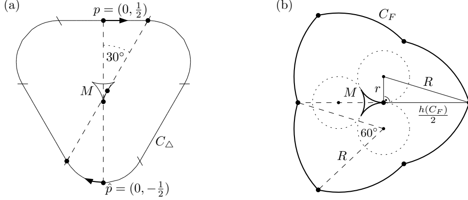
Figure 9: The “Rounded Triangle” C_\Delta and the “Flower” C_F are curves of constant halving distance.
