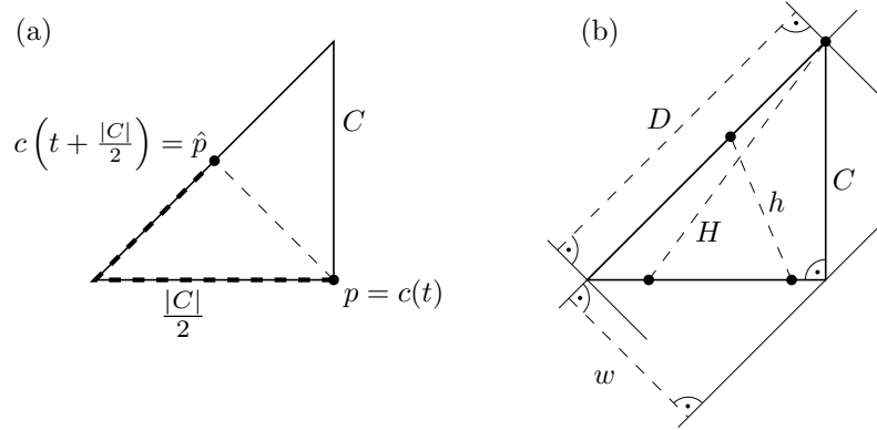
Figure 3: (a) A halving chord p\hat{p} . (b) Diameter D , width w , minimum and maximum halving distance h and H of an isosceles, right-angled triangle.
