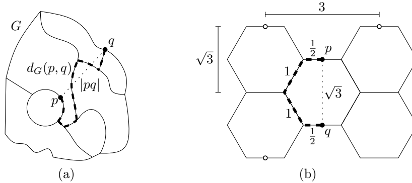
Figure 1: (a) The shortest path (dashed) between p and q in the graph G and the direct distance |pq| . (b) Three points (drawn as empty circles) embedded in a hexagonal grid with geometric dilation \sqrt{3} \approx 1.732 .
