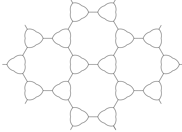
Figure 2: A section of the grid from [8] which has small dilation, less than 1.678.
