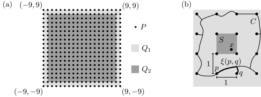
Figure 7: (a) The point set P and the square Q_2 which has to be covered by an embedding graph of low dilation. (b) Every point x \in Q_2 is encircled by a cycle of length \leq 12\delta(G) .
