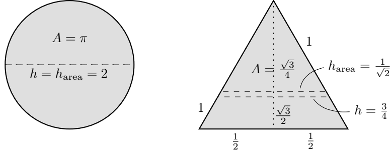
Figure 12: The equilateral triangle has a smaller ratio A/h^2 = 4/(3\sqrt{3}) \approx 0.770 and a bigger ratio A/h_{\text{area}}^2 = \sqrt{3}/2 \approx 0.866 than the circle ( \pi/4 \approx 0.785 ).
