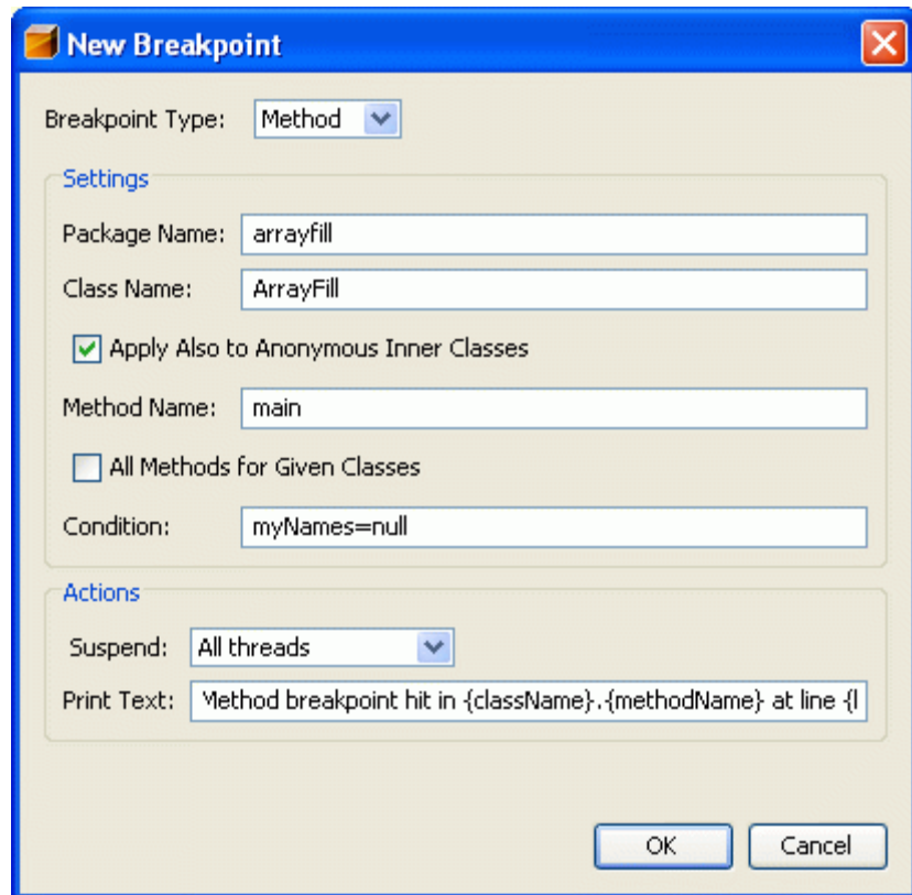
Setting a conditional breakpoint
