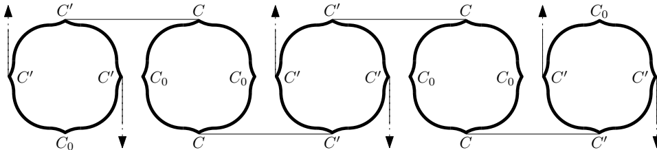
Fig. 21. Schematic view of a variable gadget with three upper and three lower exits. The pattern can be repeated arbitrarily.
