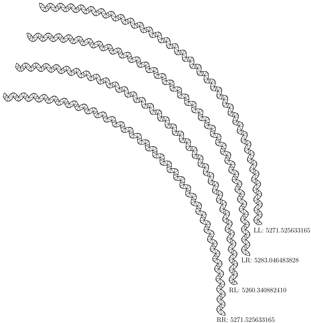
Fig. 26. Optimal solutions for all cases for the right bend
