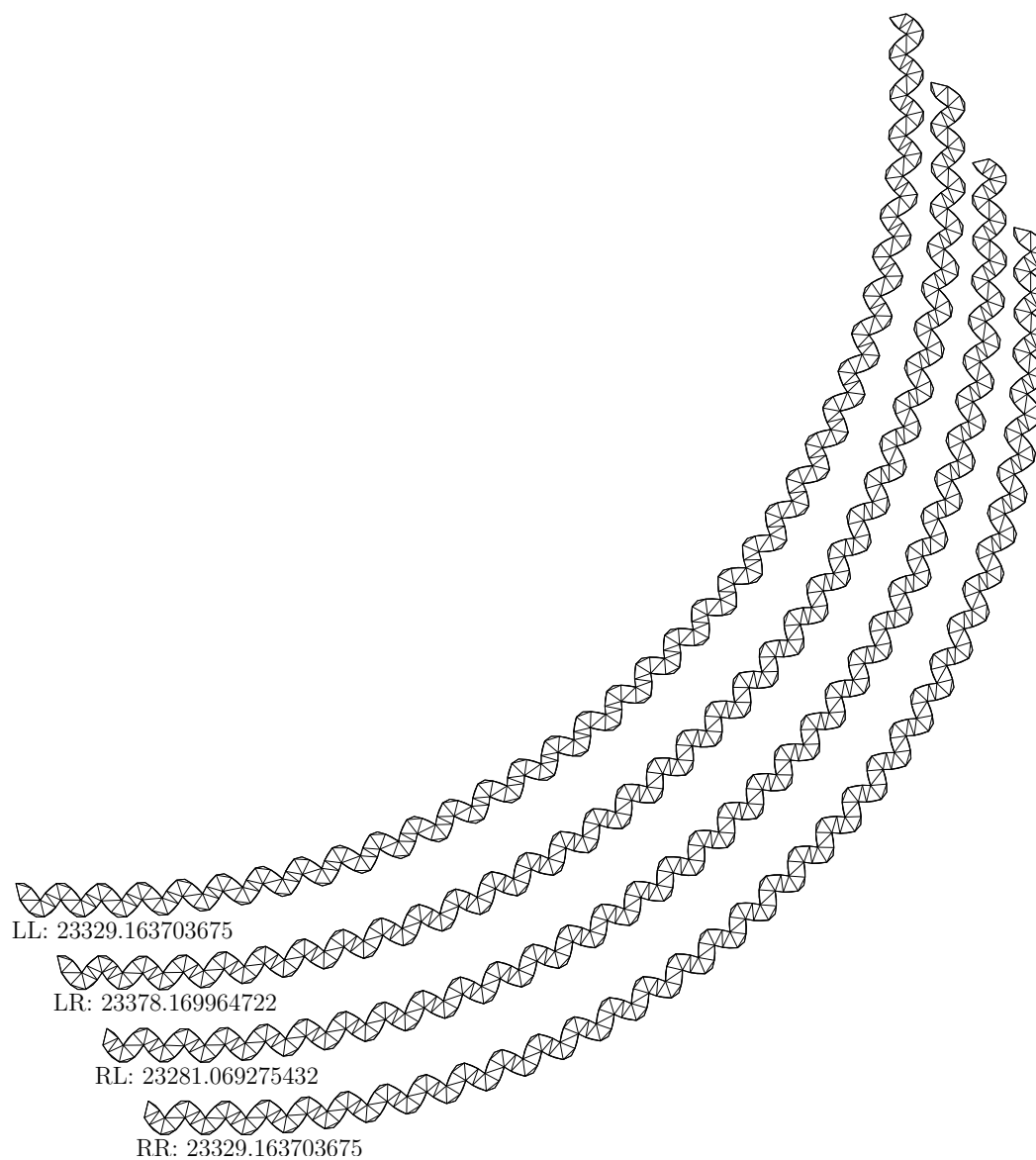
Fig. 27. Optimal solutions for all cases for the thick left bend
