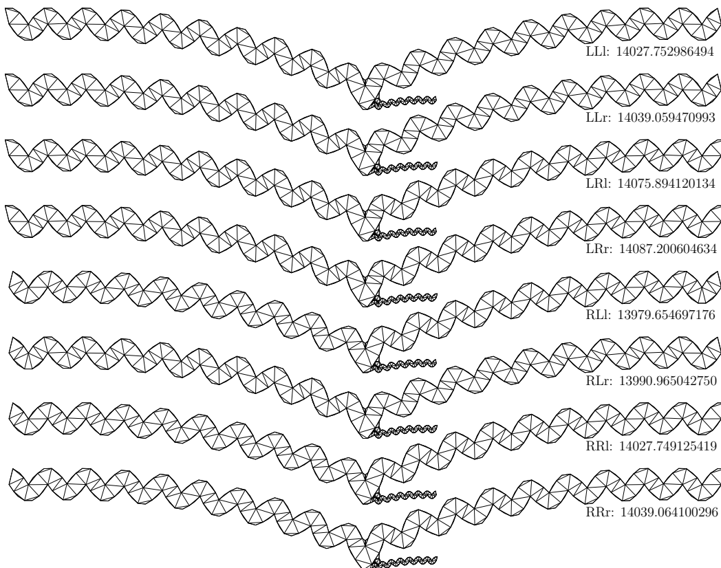
Fig. 23. Optimal solutions for all cases for the C connection
