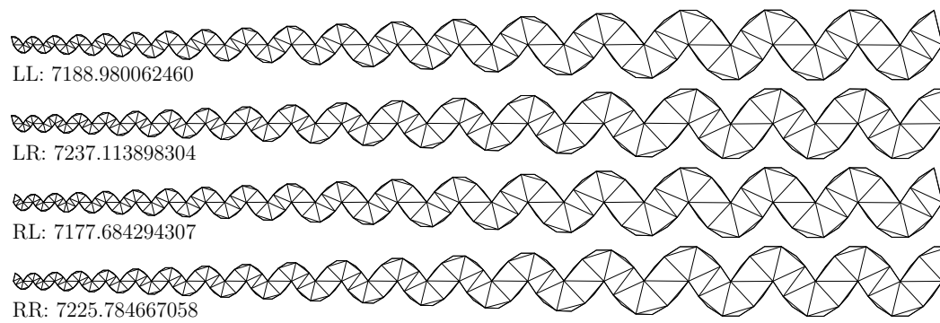
Fig. 24. Optimal solutions for all cases for the thickening adapter
