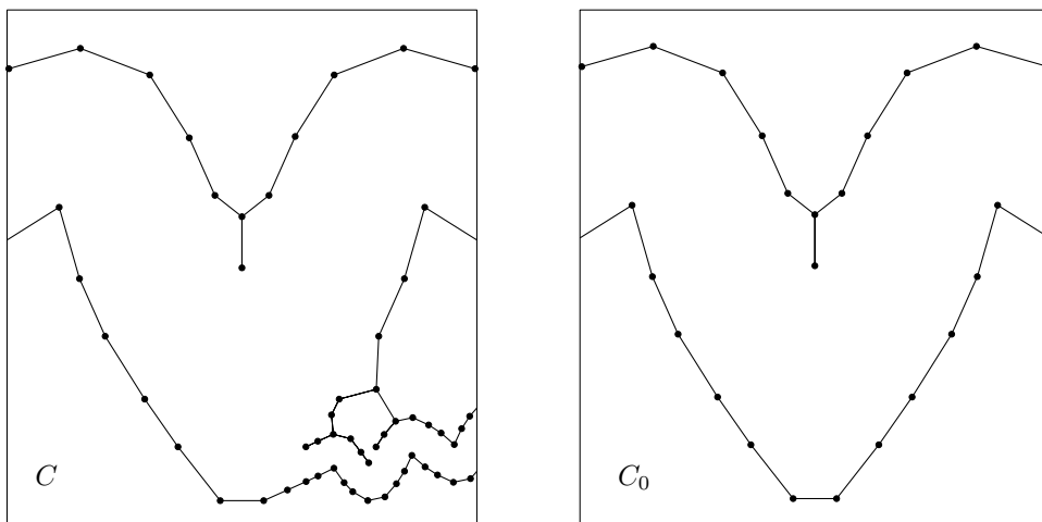
Fig. 13. Enlarged view of the central part of the C and C_0 connections.
