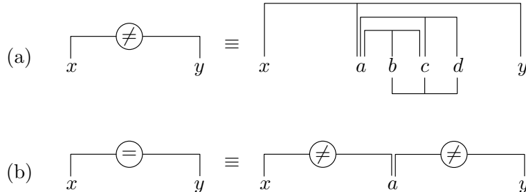
Fig. 5. The gadgets to enforce inequality (a) and equality (b) between two variables.
