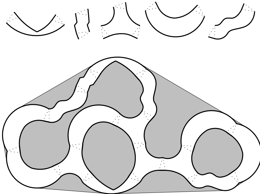
Fig. 3. A schematic view of the construction: From the five types of building blocks shown at the top, one can build a network of tubes like in the lower part. The area within this network is the interesting part where the simulation of the logic takes place. The holes inside the structure and the pockets between the structure and the convex hull (drawn shaded) form simple polygons that can be optimally triangulated in polynomial time.
