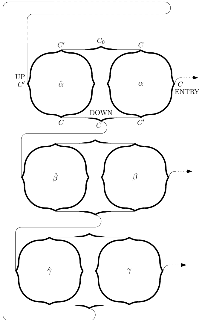
Fig. 20. Schematic view of the clause gadget. The dashed parts of the wires are long enough for sufficiently many copies of the wire-piece and the extended wire-piece to ensure that the wire can reach from the lowest C connection to the left C' connection of \hat{\alpha} (Lemma 6.1).
