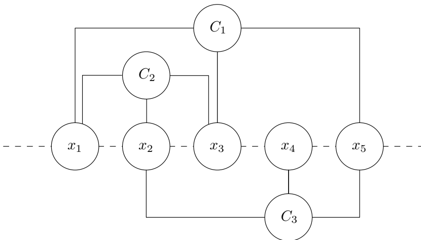
Fig. 4. A rectilinear embedding of graph that is associated with the Boolean formula (x_1 \vee \neg x_3 \vee x_5) \wedge (\neg x_1 \vee x_2 \vee x_3) \wedge (x_2 \vee x_4 \vee \neg x_5) .
