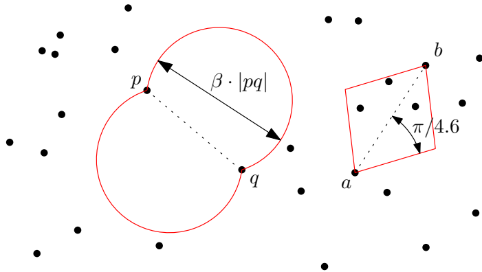
Fig. 8. An edge pq of the \beta -skeleton. The edge ab does not belong to the MWT since the diamond test is violated.
