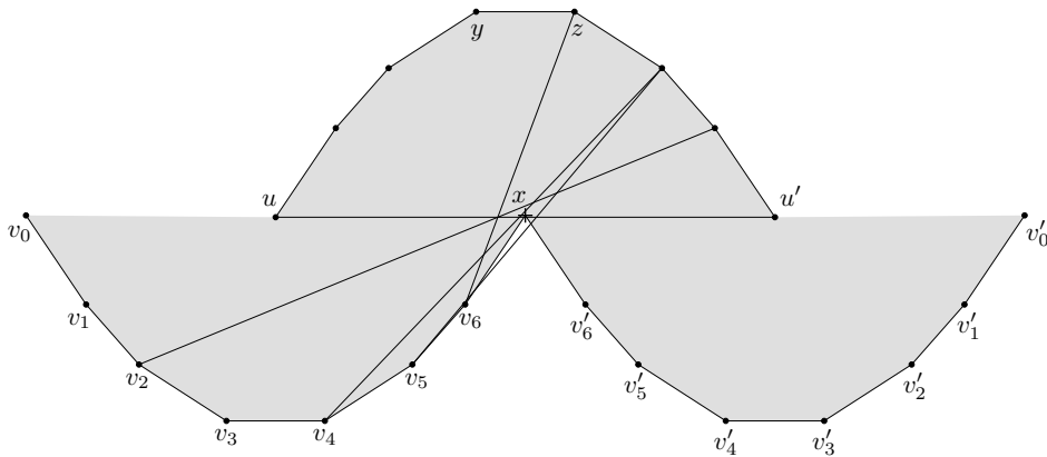
Fig. 10. The point set W in Lemma 5.1 is in sufficiently general position.
