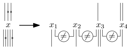
Fig. 6. Getting rid of negations: The variable x in this example has eight connections, some of which are negated, as indicated by crosses. We replace x by a chain of variables x_1, x_2, \dots with alternating truth values and place the connections to the clauses containing x correspondingly.
