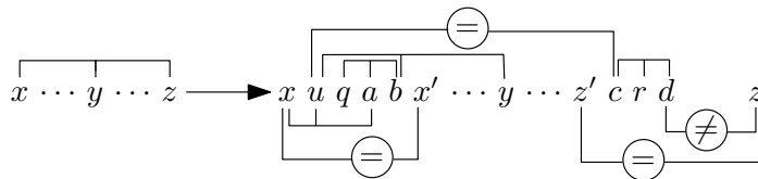
Fig. 7. The modification for a clause x \vee y \vee z with three literals.
