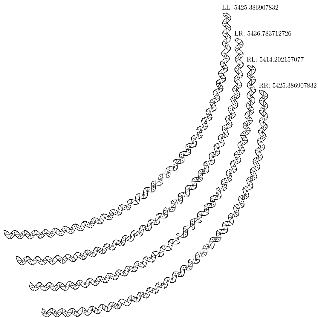
Fig. 25. Optimal solutions for all cases for the left bend
