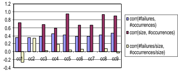
Figure 6. Correlations needed to determine the interesting sets of code constructs.
